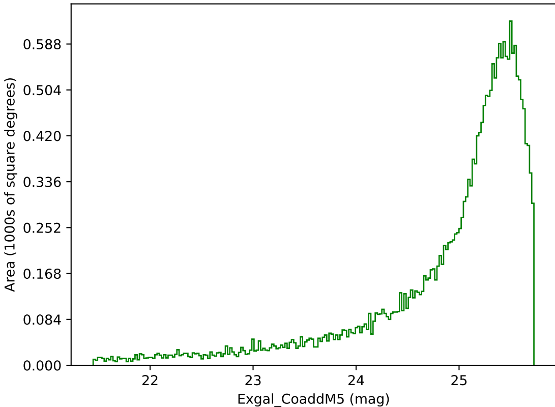
weather_cloudso36v3.4_10yrs Yr 1 g band: Exgal_CoaddM5
