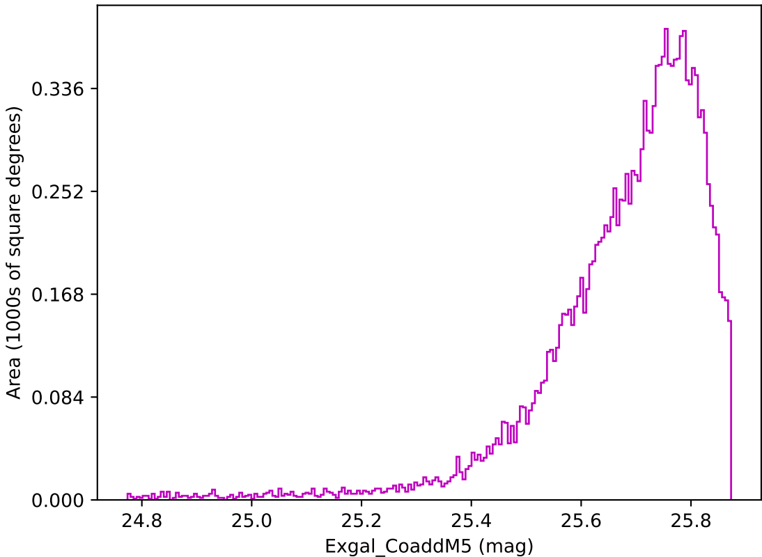
weather_cloudso36v3.4_10yrs WFD z band: Exgal_CoaddM5
