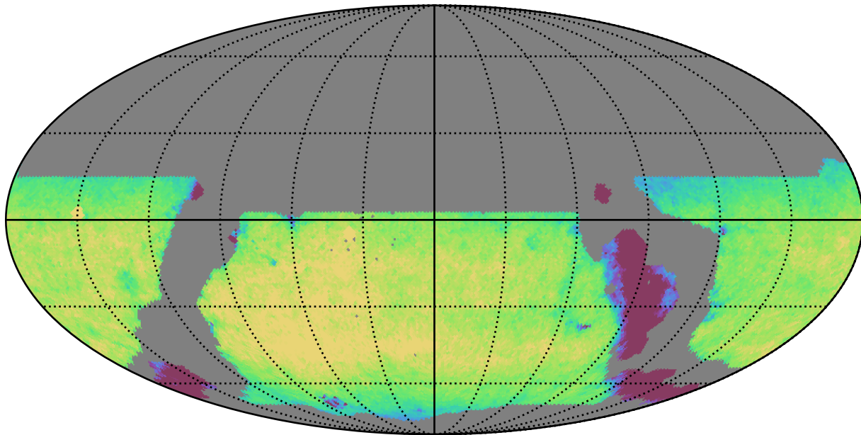
weather_cloudso36v3.4_10yrs WFD y band: Exgal_CoaddM5
