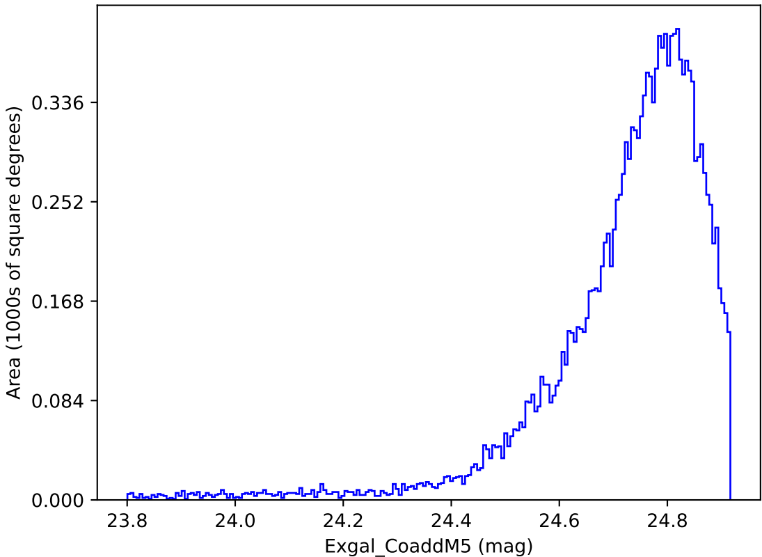
weather_cloudso36v3.4_10yrs WFD y band: Exgal_CoaddM5
