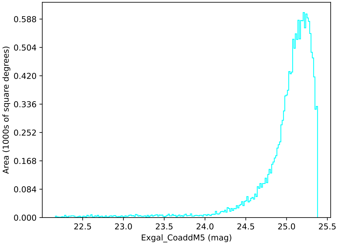
weather_cloudso36v3.4_10yrs WFD u band: Exgal_CoaddM5
