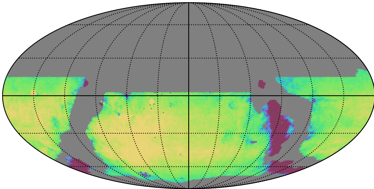
weather_cloudso36v3.4_10yrs WFD r band: Exgal_CoaddM5
