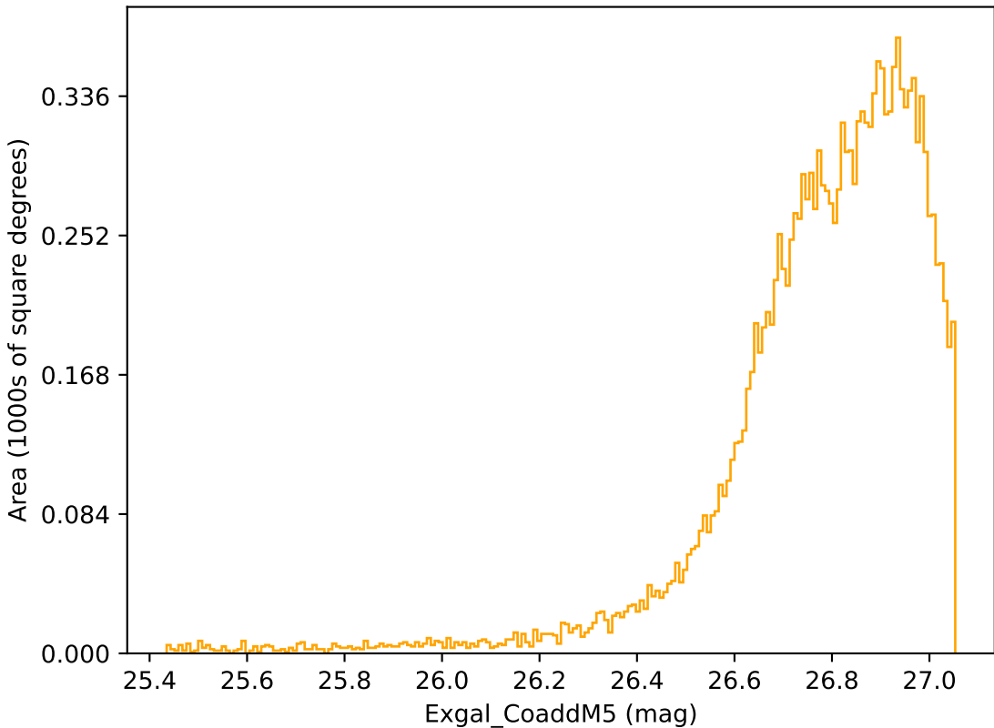
weather_cloudso36v3.4_10yrs WFD r band: Exgal_CoaddM5
