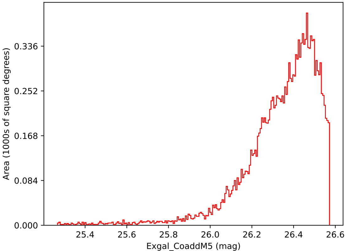
weather_cloudso36v3.4_10yrs WFD i band: Exgal_CoaddM5
