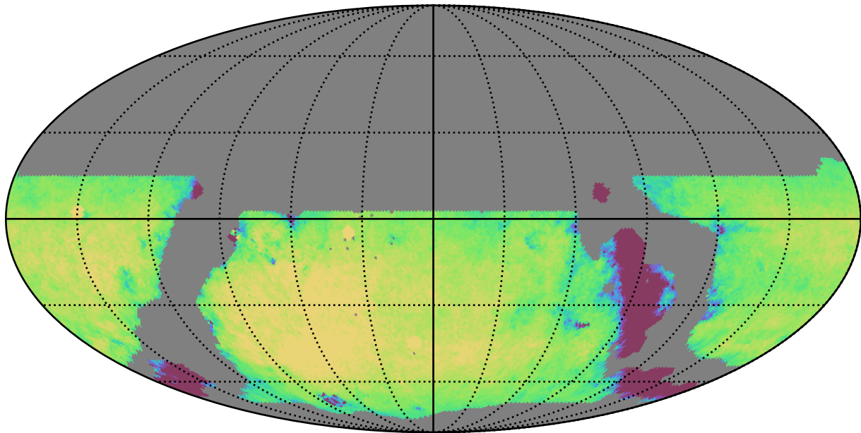
weather_cloudso36v3.4_10yrs WFD g band: Exgal_CoaddM5
