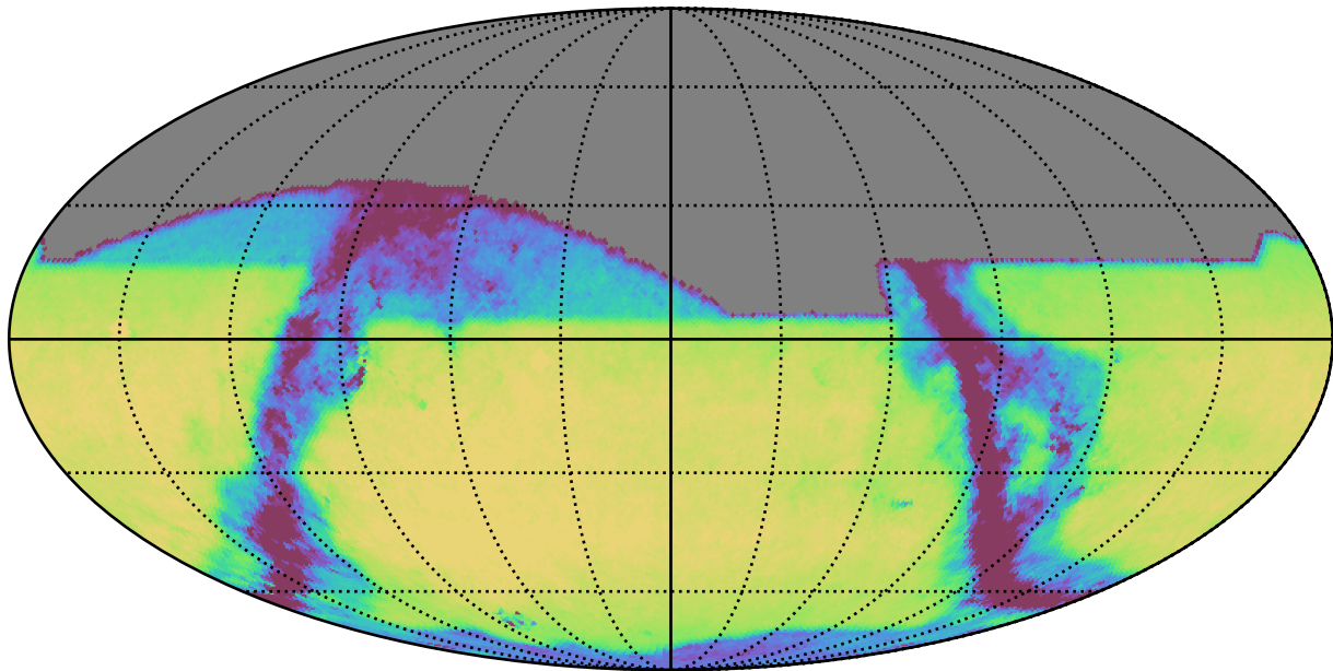
weather_cloudso36v3.4_10yrs All sky z band: Exgal_CoaddM5
