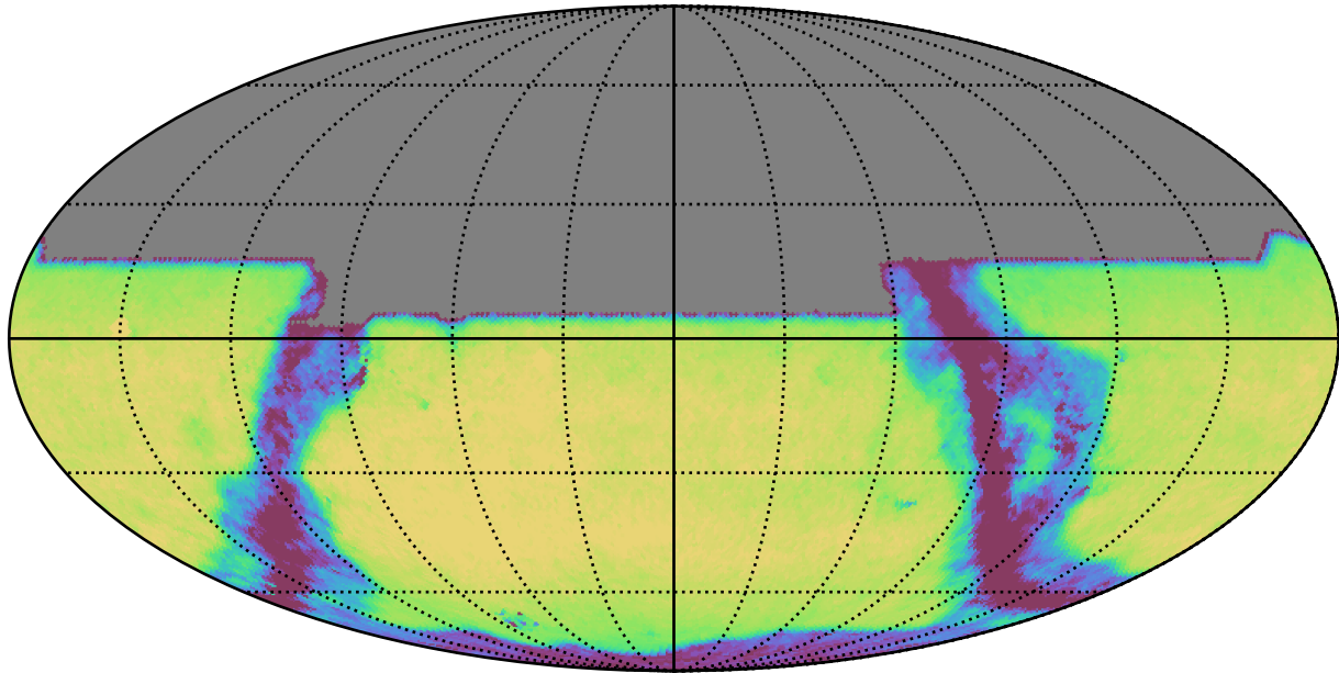
weather_cloudso36v3.4_10yrs All sky y band: Exgal_CoaddM5
