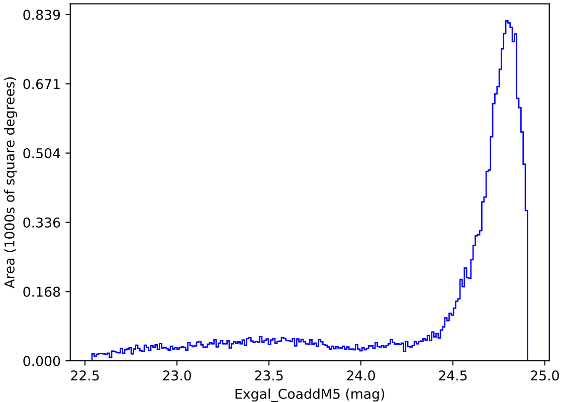
weather_cloudso36v3.4_10yrs All sky y band: Exgal_CoaddM5
