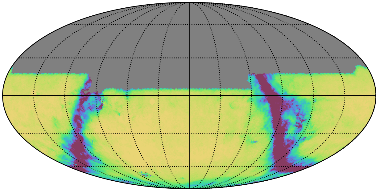
weather_cloudso36v3.4_10yrs All sky u band: Exgal_CoaddM5
