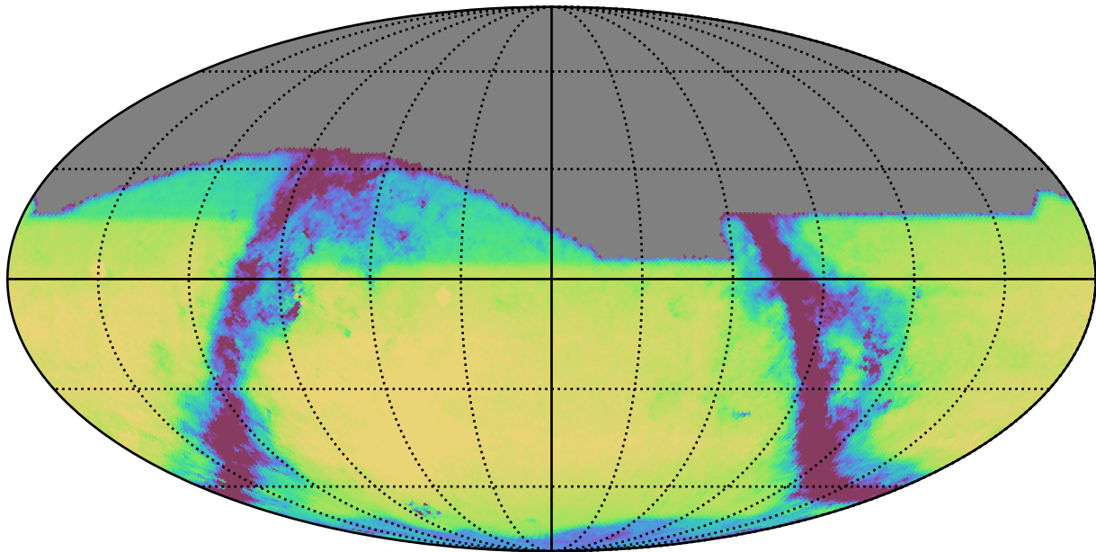
weather_cloudso36v3.4_10yrs All sky r band: Exgal_CoaddM5
