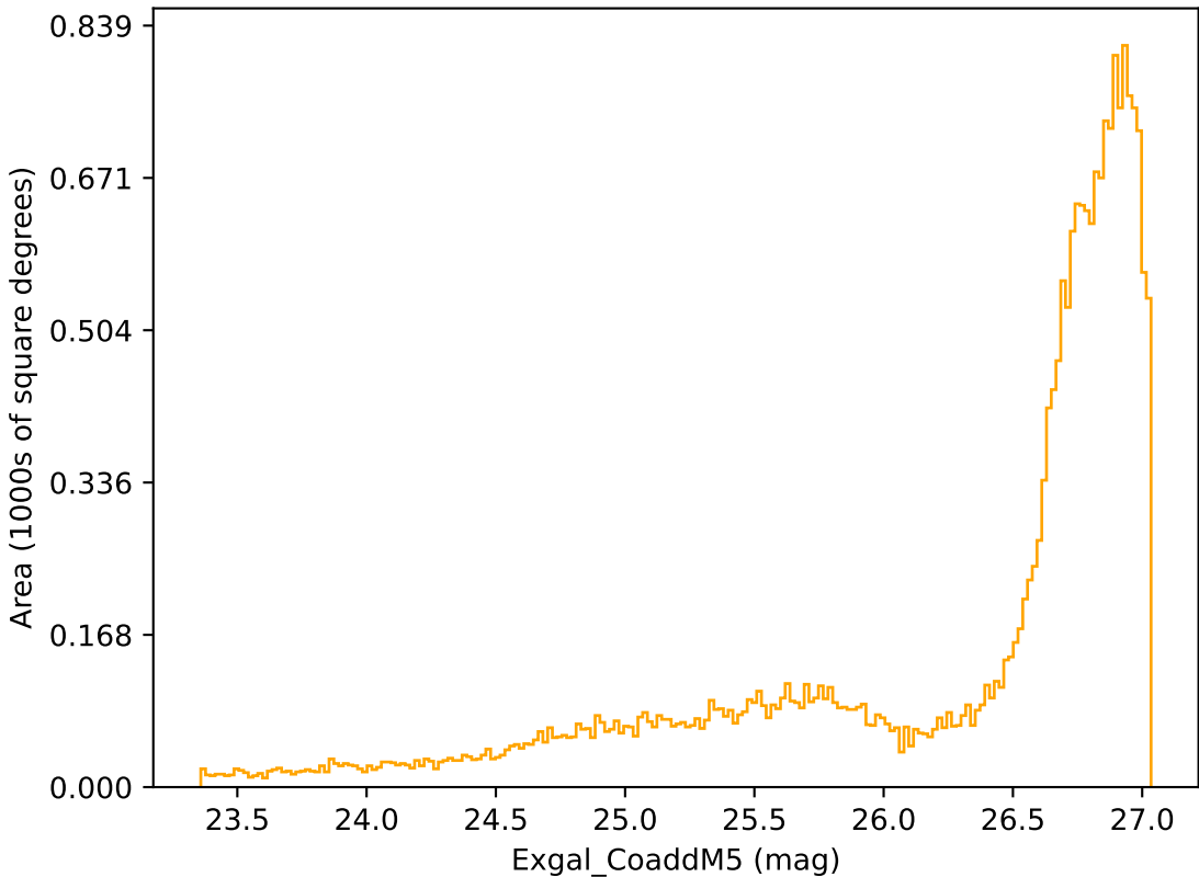
weather_cloudso36v3.4_10yrs All sky r band: Exgal_CoaddM5
