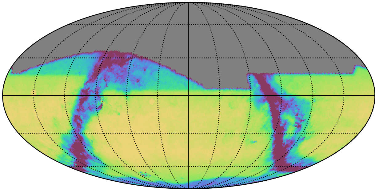
weather_cloudso36v3.4_10yrs All sky i band: Exgal_CoaddM5
