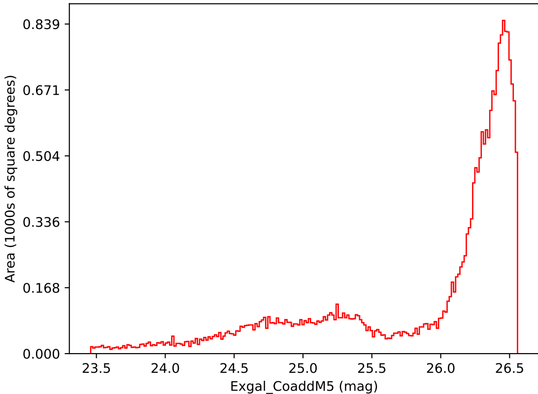
weather_cloudso36v3.4_10yrs All sky i band: Exgal_CoaddM5
