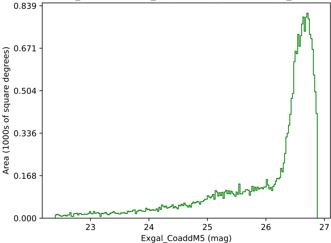
weather_cloudso36v3.4_10yrs All sky g band: Exgal_CoaddM5
