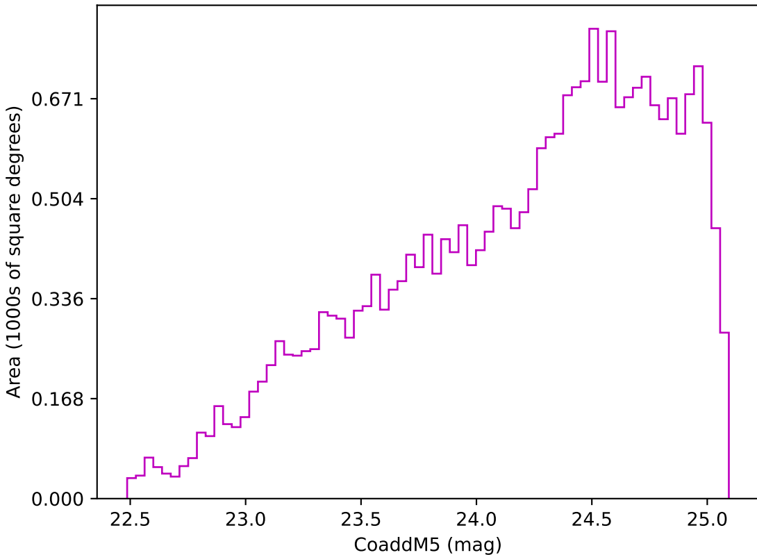
weather_cloudso36v3.4_10yrs Yr 3-4 z band: CoaddM5
