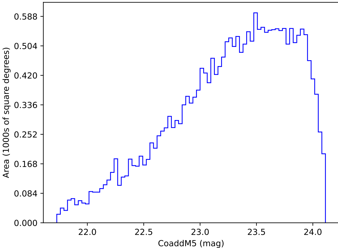
weather_cloudso36v3.4_10yrs Yr 3-4 y band: CoaddM5
