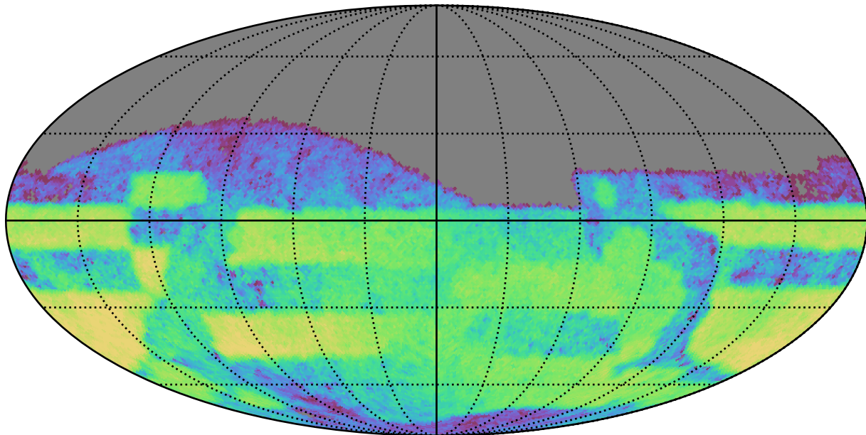
weather_cloudso36v3.4_10yrs Yr 3-4 r band: CoaddM5
