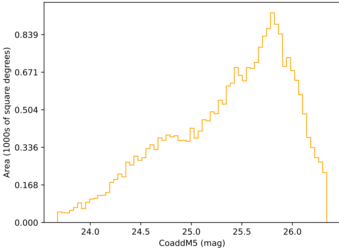
weather_cloudso36v3.4_10yrs Yr 3-4 r band: CoaddM5
