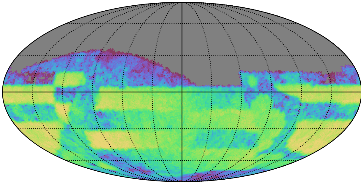
weather_cloudso36v3.4_10yrs Yr 3-4 i band: CoaddM5
