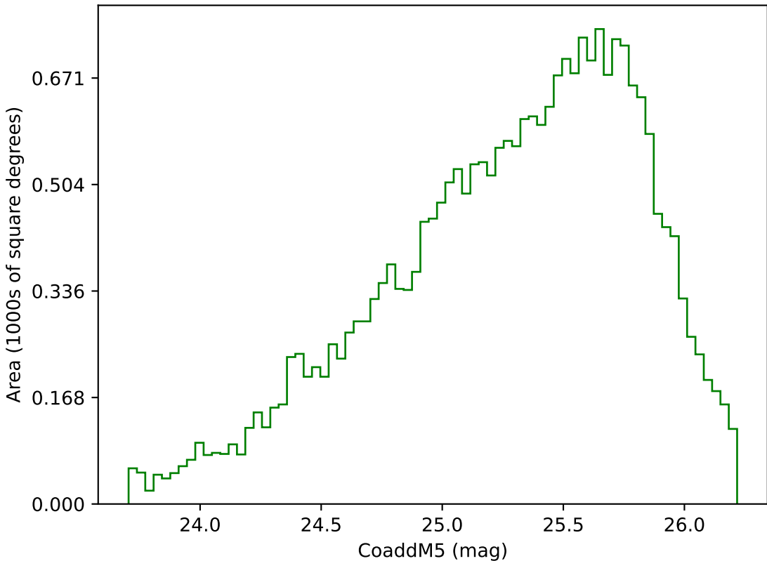
weather_cloudso36v3.4_10yrs Yr 3-4 g band: CoaddM5
