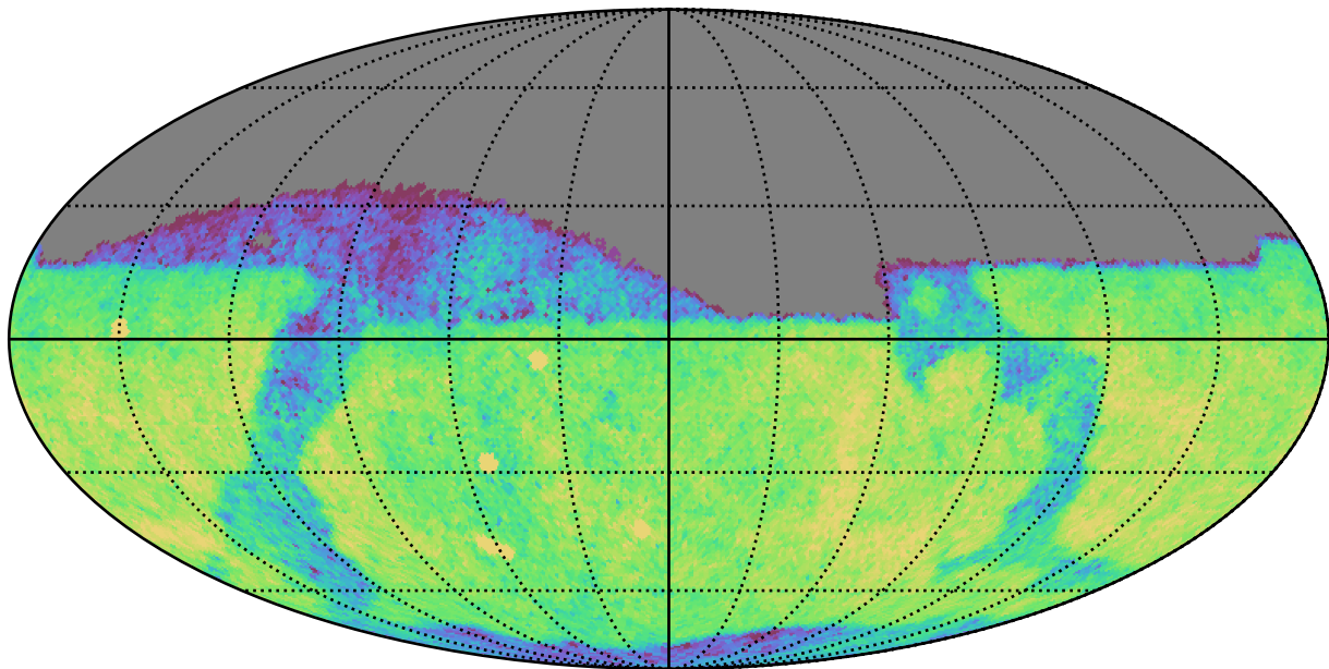
weather_cloudso36v3.4_10yrs Yr 1 z band: CoaddM5
