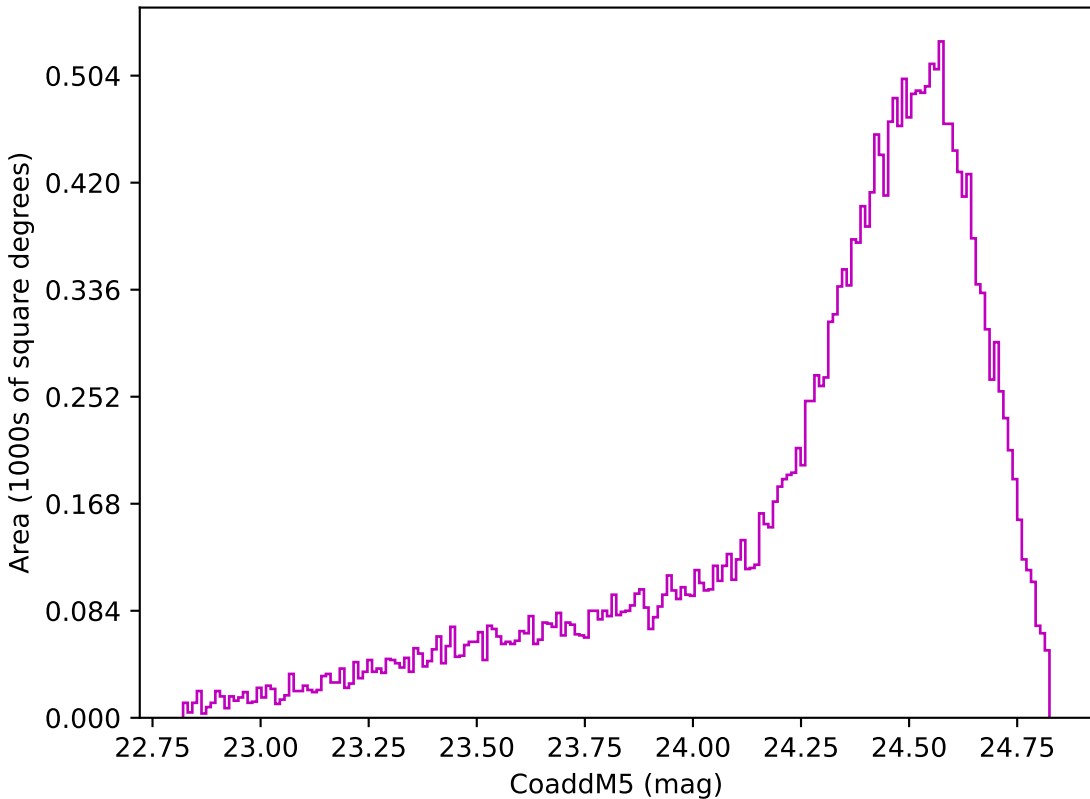
weather_cloudso36v3.4_10yrs Yr 1 z band: CoaddM5
