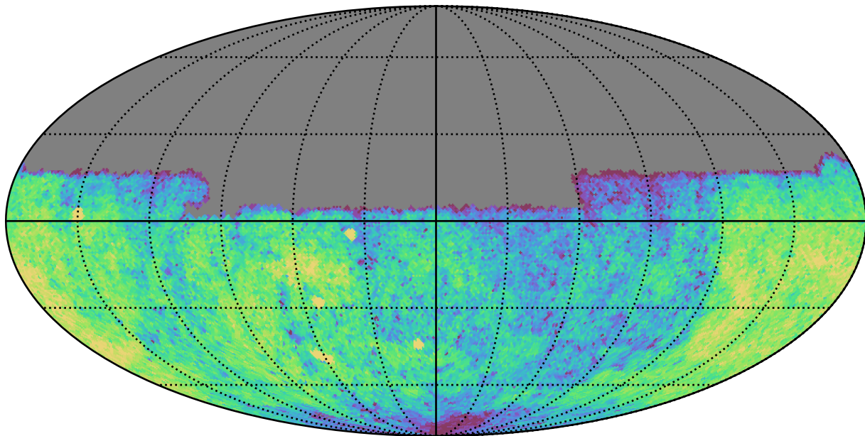
weather_cloudso36v3.4_10yrs Yr 1 u band: CoaddM5
