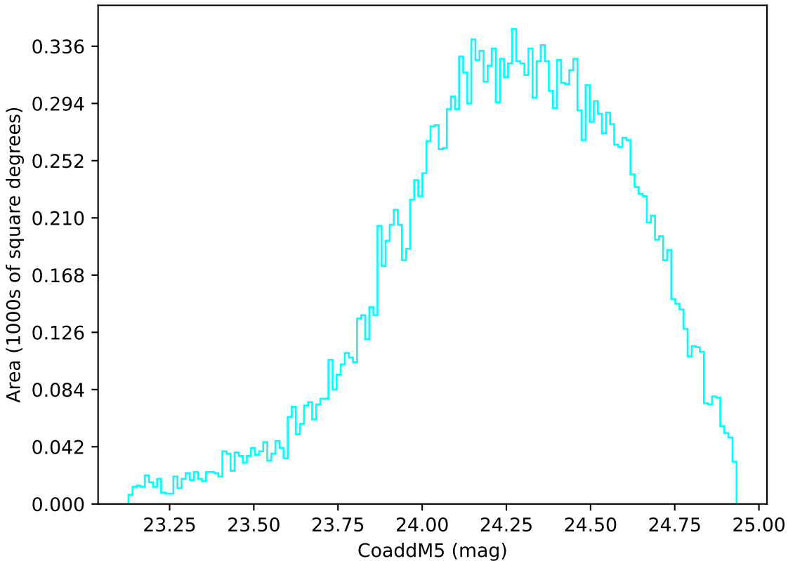
weather_cloudso36v3.4_10yrs Yr 1 u band: CoaddM5
