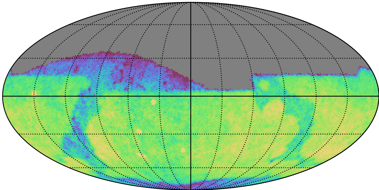
weather_cloudso36v3.4_10yrs Yr 1 r band: CoaddM5
