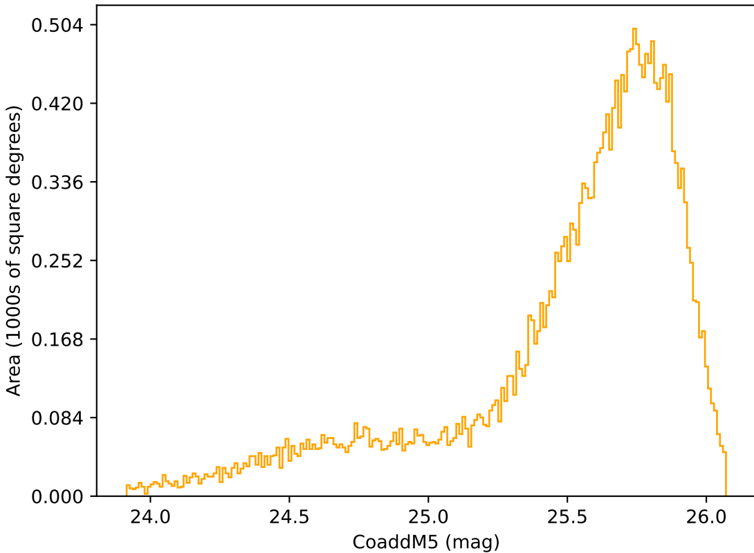
weather_cloudso36v3.4_10yrs Yr 1 r band: CoaddM5
