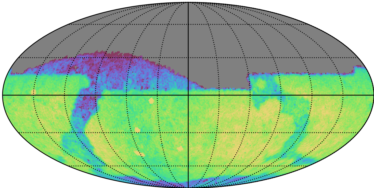
weather_cloudso36v3.4_10yrs Yr 1 i band: CoaddM5
