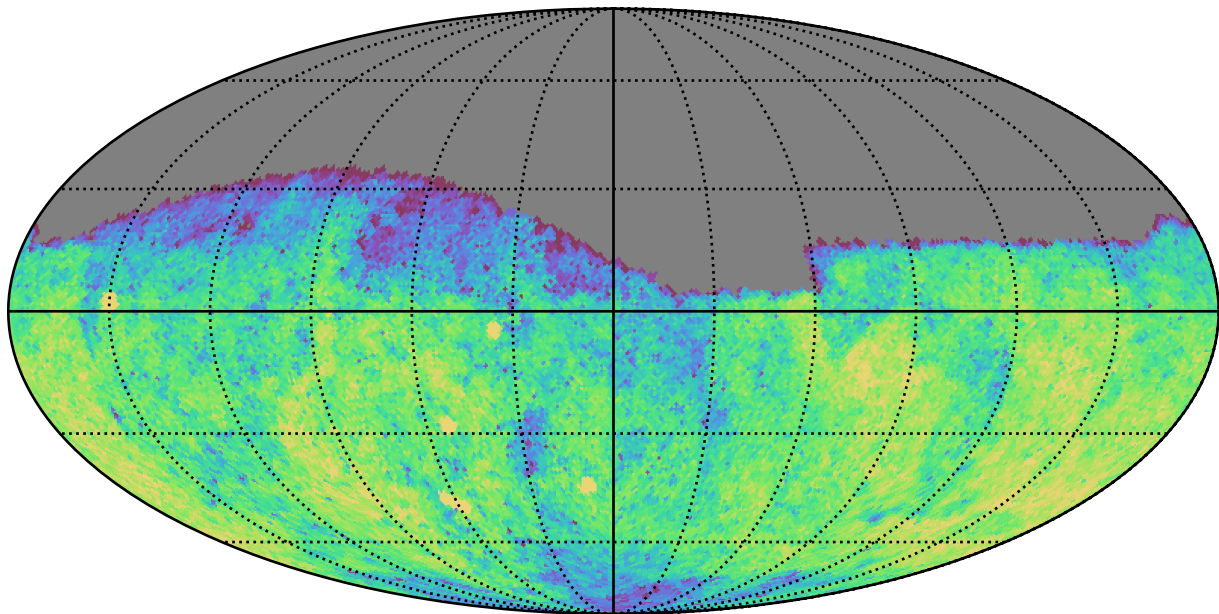
weather_cloudso36v3.4_10yrs Yr 1 g band: CoaddM5
