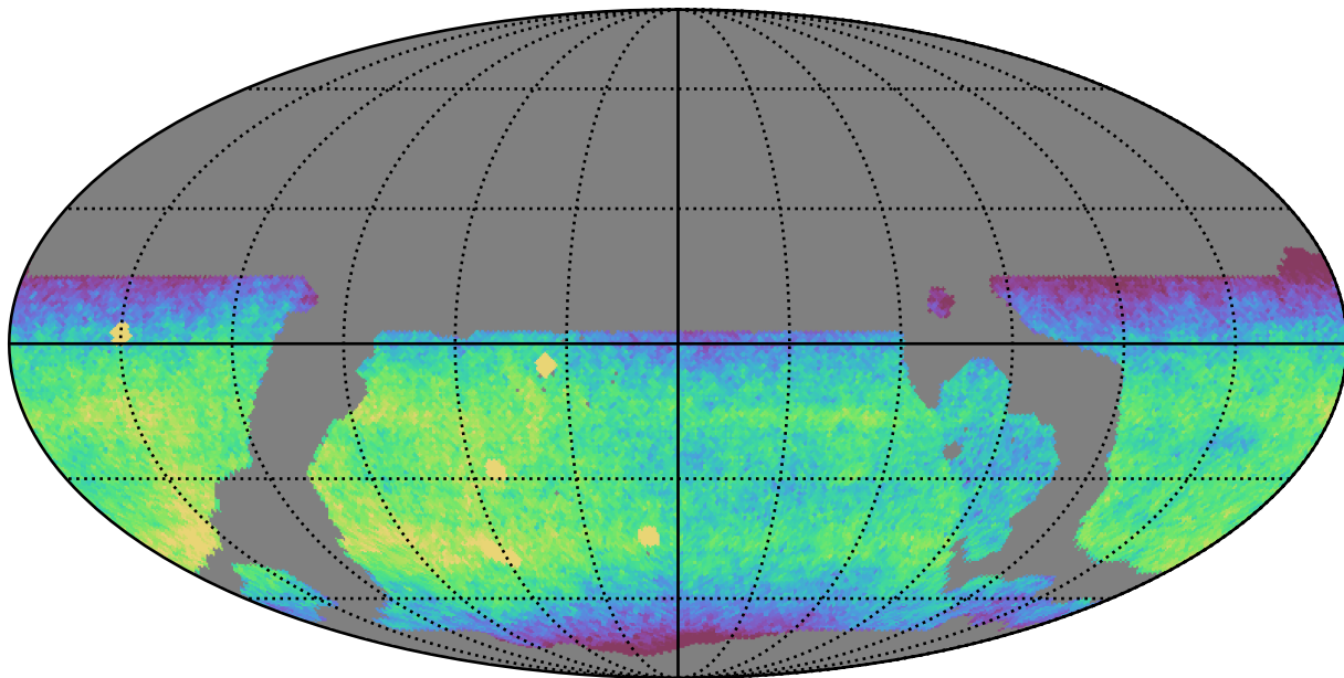
weather_cloudso36v3.4_10yrs WFD z band: CoaddM5
