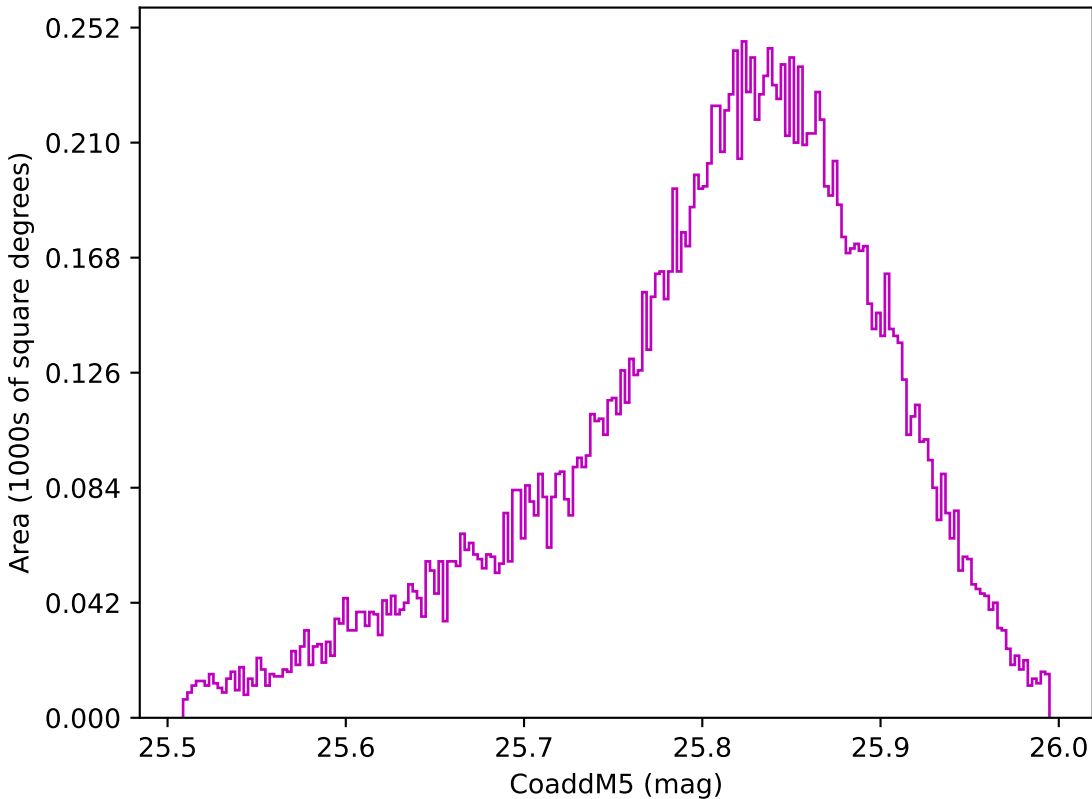
weather_cloudso36v3.4_10yrs WFD z band: CoaddM5
