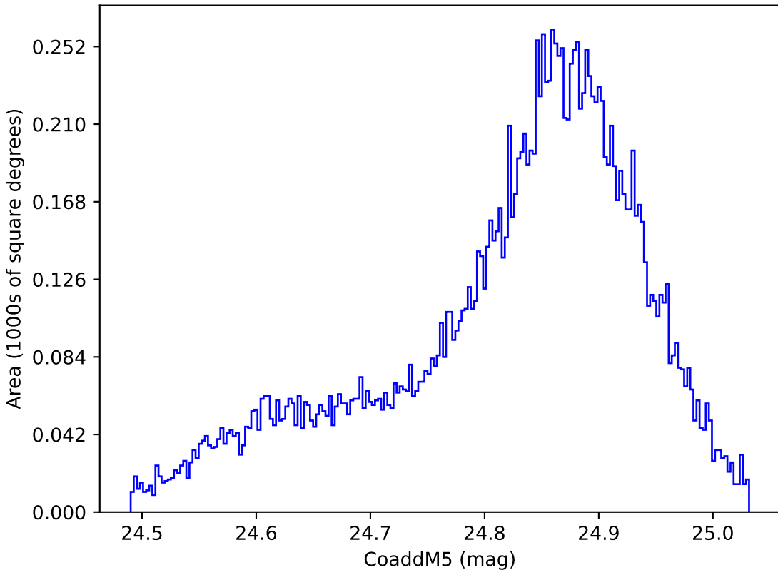
weather_cloudso36v3.4_10yrs WFD y band: CoaddM5
