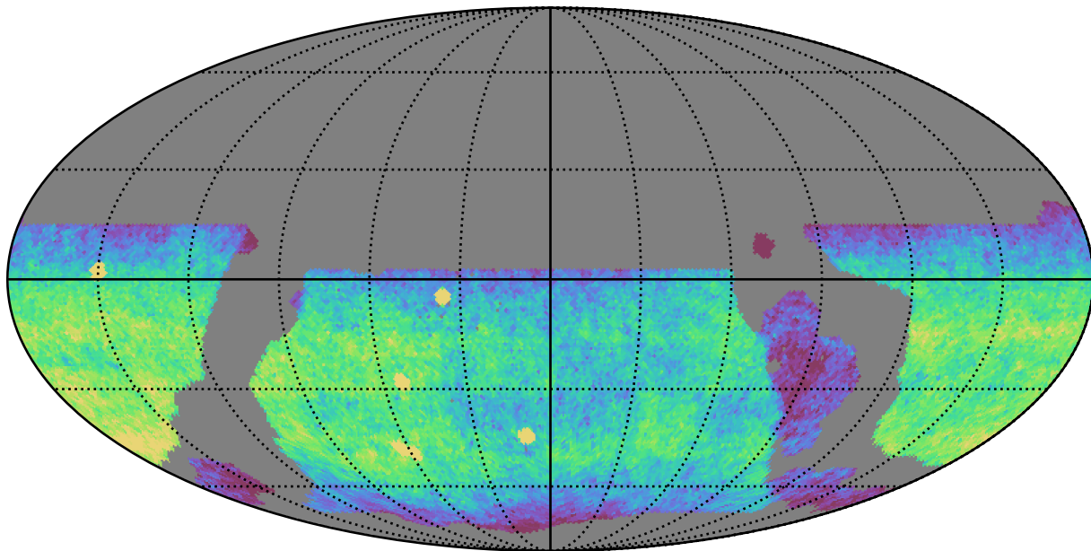
weather_cloudso36v3.4_10yrs WFD u band: CoaddM5
