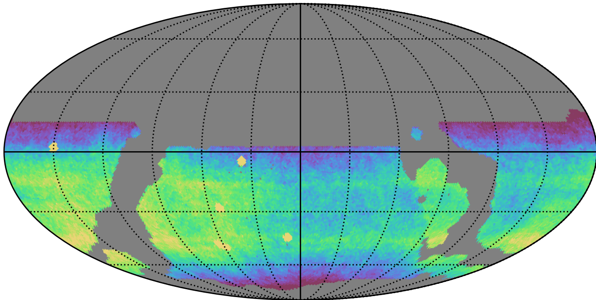
weather_cloudso36v3.4_10yrs WFD r band: CoaddM5
