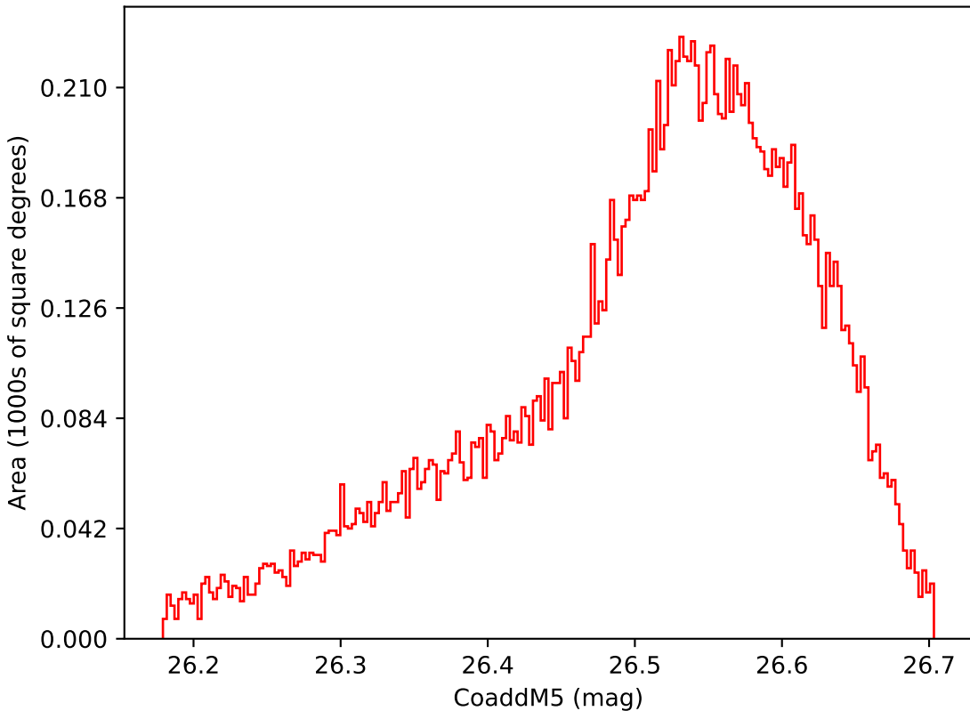
weather_cloudso36v3.4_10yrs WFD i band: CoaddM5
