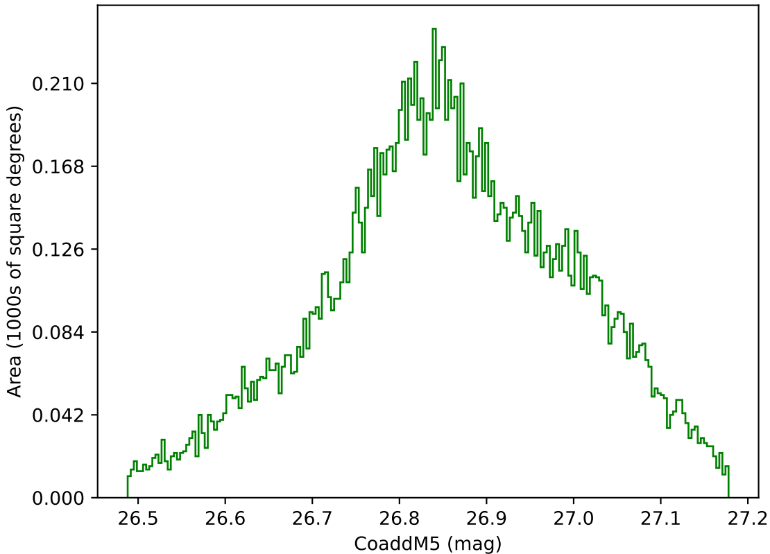
weather_cloudso36v3.4_10yrs WFD g band: CoaddM5
