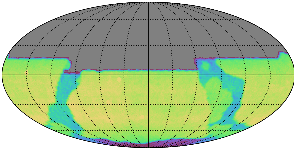
weather_cloudso36v3.4_10yrs All sky y band: CoaddM5
