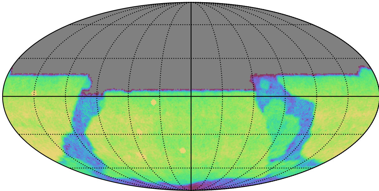
weather_cloudso36v3.4_10yrs All sky u band: CoaddM5
