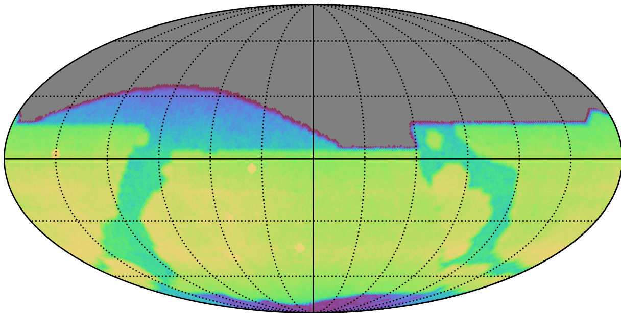
weather_cloudso36v3.4_10yrs All sky r band: CoaddM5
