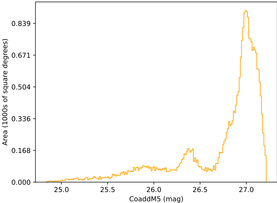
weather_cloudso36v3.4_10yrs All sky r band: CoaddM5
