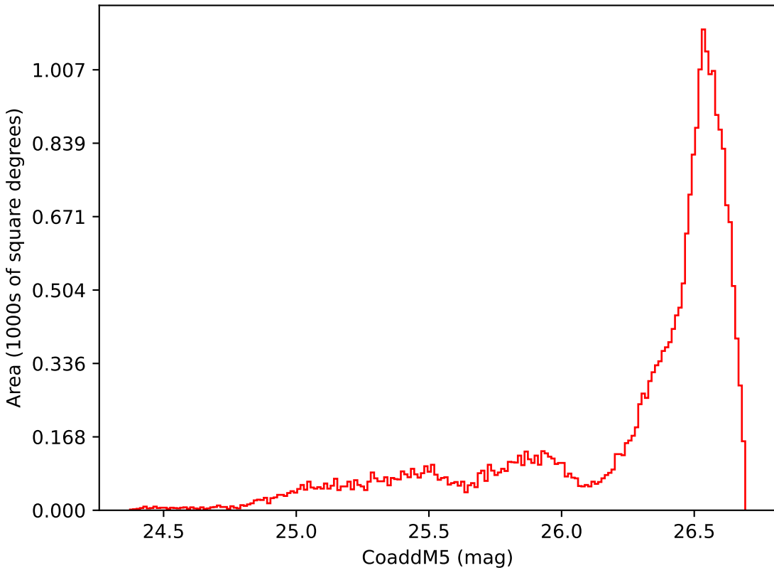
weather_cloudso36v3.4_10yrs All sky i band: CoaddM5
