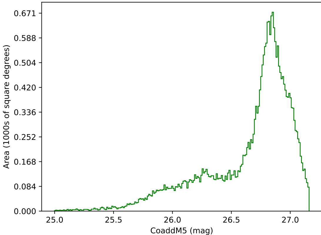
weather_cloudso36v3.4_10yrs All sky g band: CoaddM5
