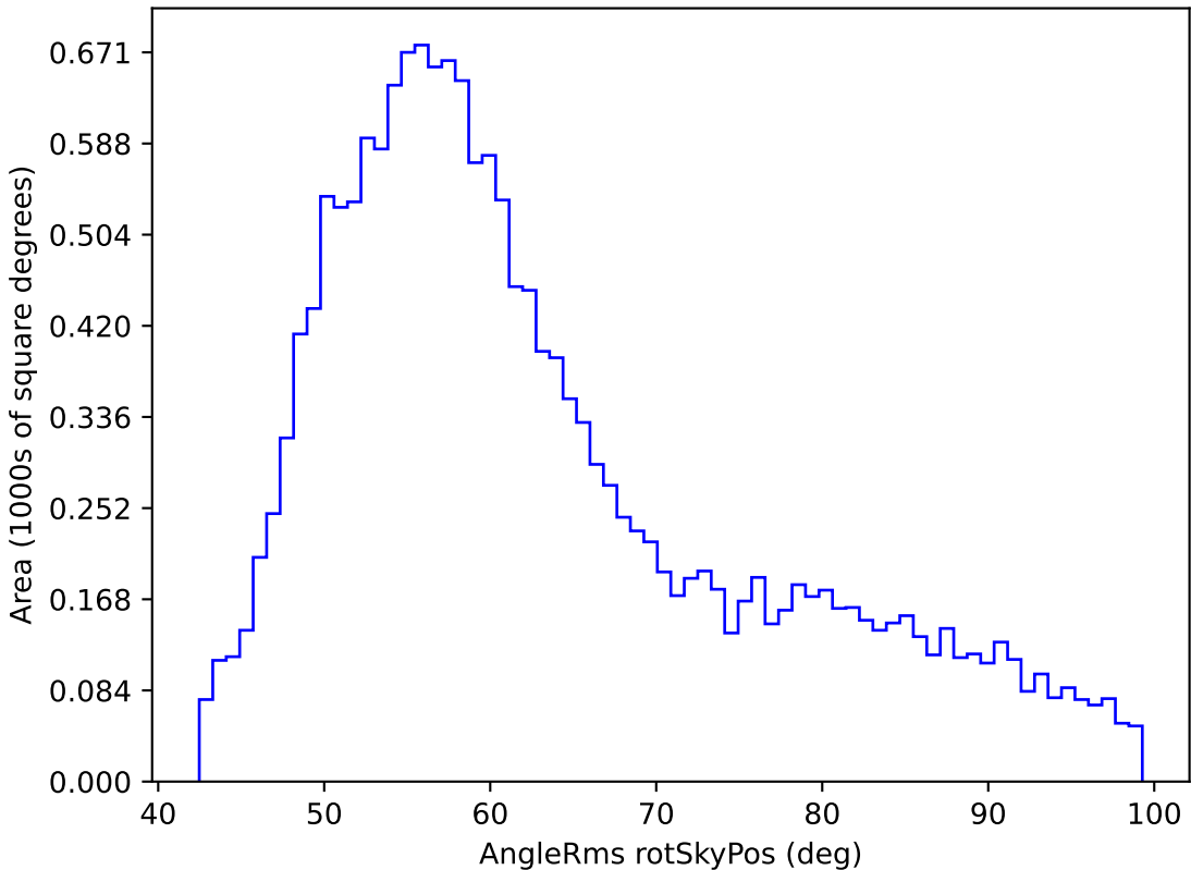
weather_cloudso36v3.4_10yrs WFD u band: AngleRms rotSkyPos
