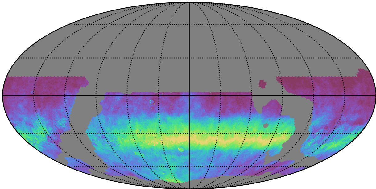
weather_cloudso36v3.4_10yrs WFD r band: AngleRms rotSkyPos
