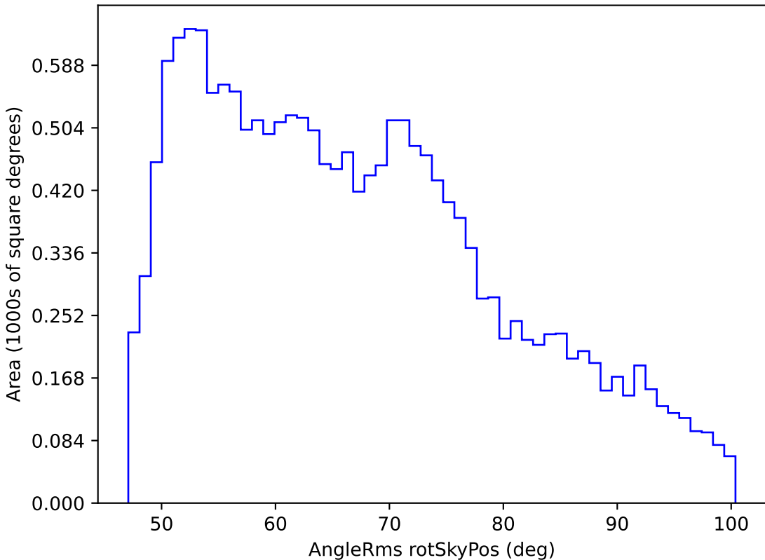
weather_cloudso36v3.4_10yrs WFD r band: AngleRms rotSkyPos
