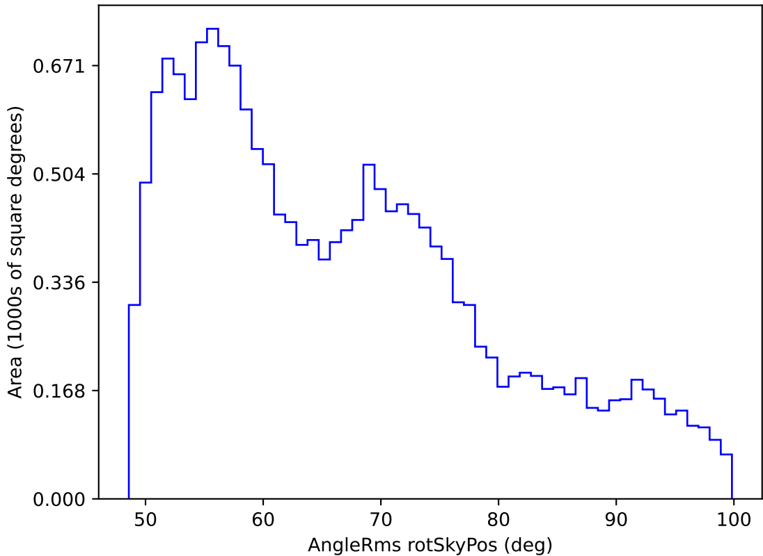
weather_cloudso36v3.4_10yrs WFD all bands: AngleRms rotSkyPos
