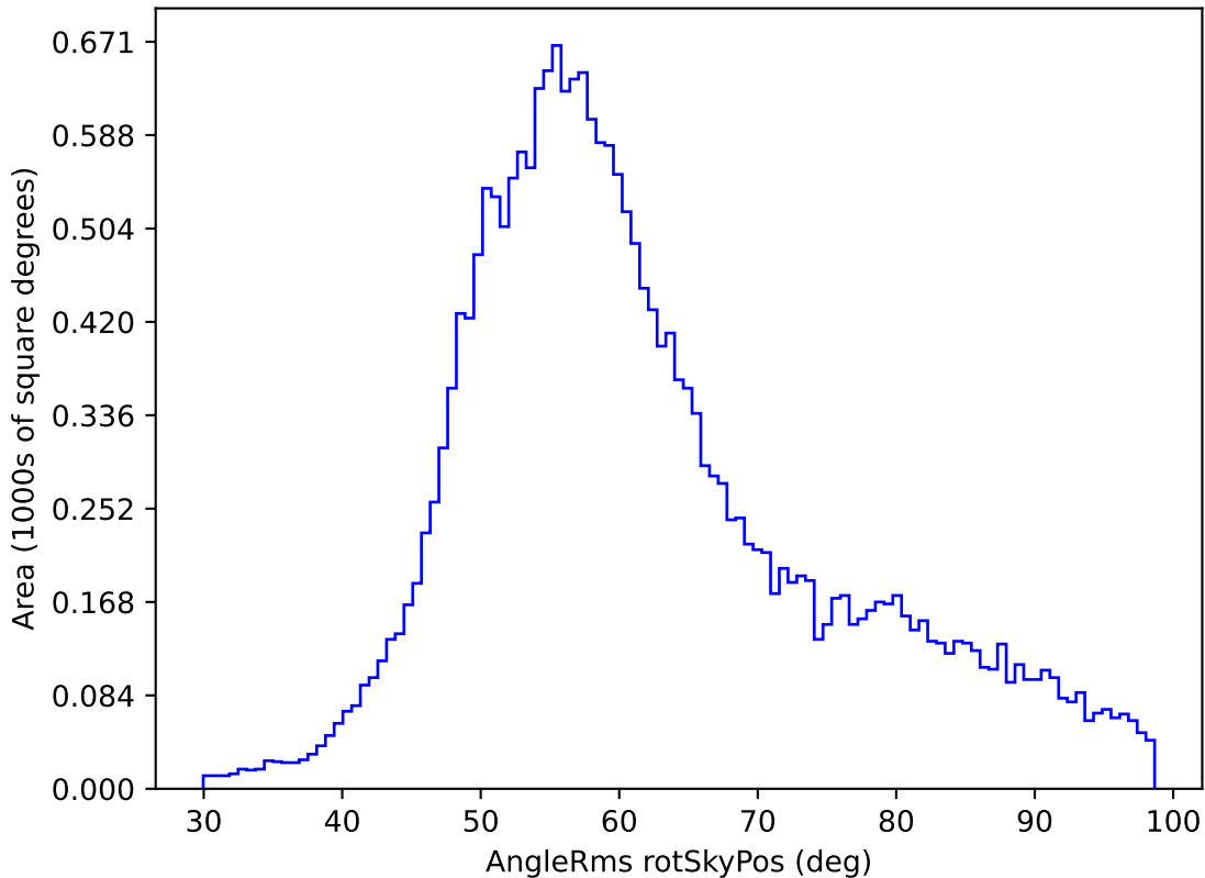
weather_cloudso36v3.4_10yrs All sky u band: AngleRms rotSkyPos
